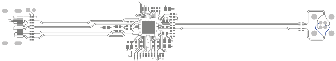
Figure 34. DS90UH949-Q1 Serializer Layout Example
