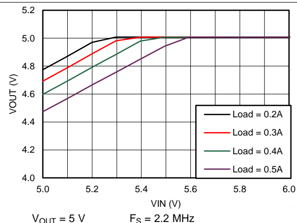
Figure 80. Dropout Curve
