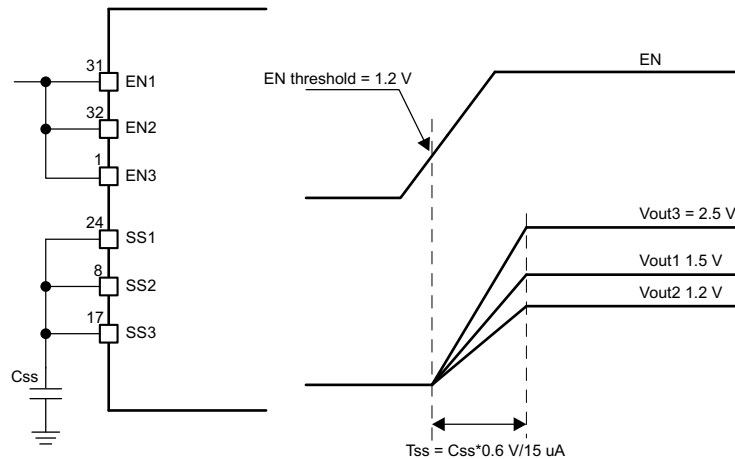
图 8-6. Ratiometric Power-Up Using SSx Pins
