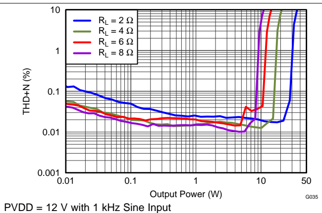
Figure 29. THD+N vs Output Power
