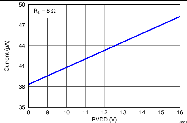
Figure 13. Shutdown Current Draw vs PVDD (Filterless)
