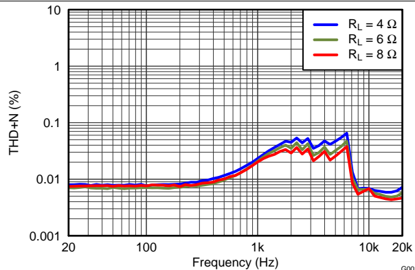
PVDD = 12 V, P_{\text{OSPK}} = 1 \text{ W} Figure 16. THD+N vs Frequency
