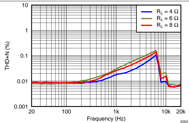
PVDD = 12 V, P_{\text{OSPK}} = 1 \text{ W} Figure 15. THD+N vs Frequency
