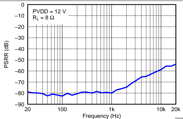
Figure 9. PVDD PSRR vs Frequency
