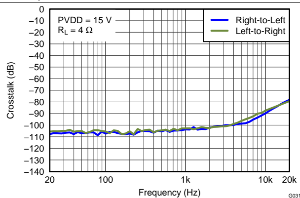
Figure 8. Crosstalk vs Frequency
