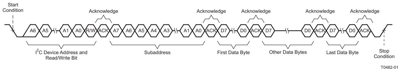
Figure 13. Multiple-Byte Write Transfer
