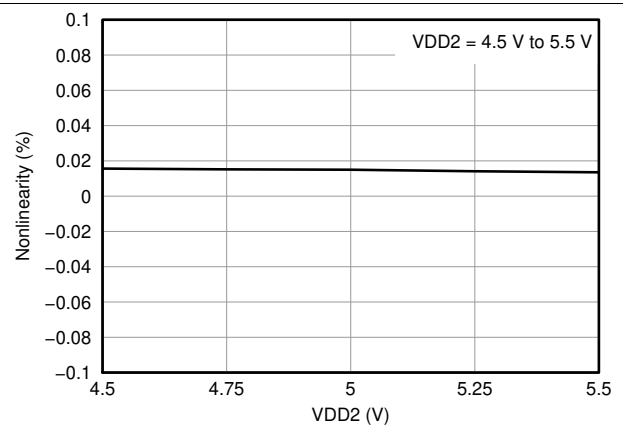
Figure 18. Nonlinearity vs High-Side Supply Voltage
