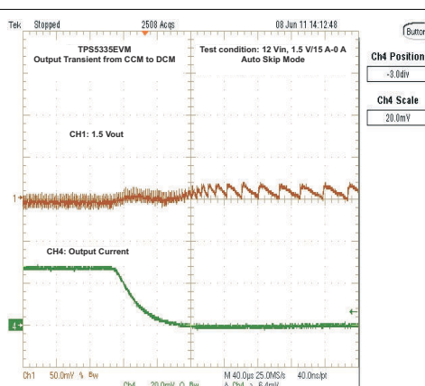
图 8-6. Output Transient From CCM to DCM
