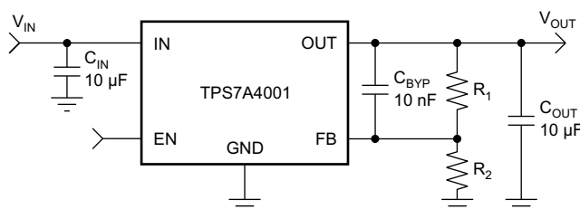
Figure 13. Adjustable Operation for Maximum AC Performance
