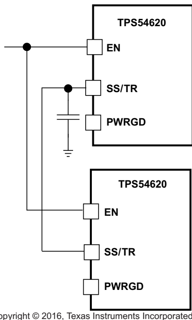
Figure 28. Ratiometric Start Up Sequence
