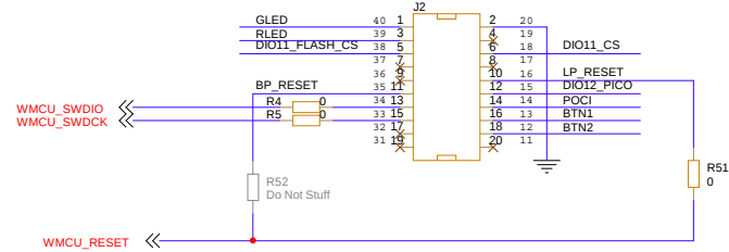
5V and 3V headers
