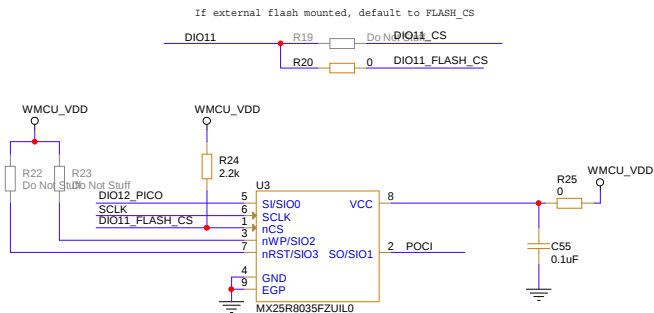
External flash
