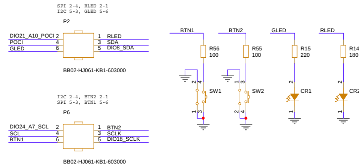
Buttons / LEDs
