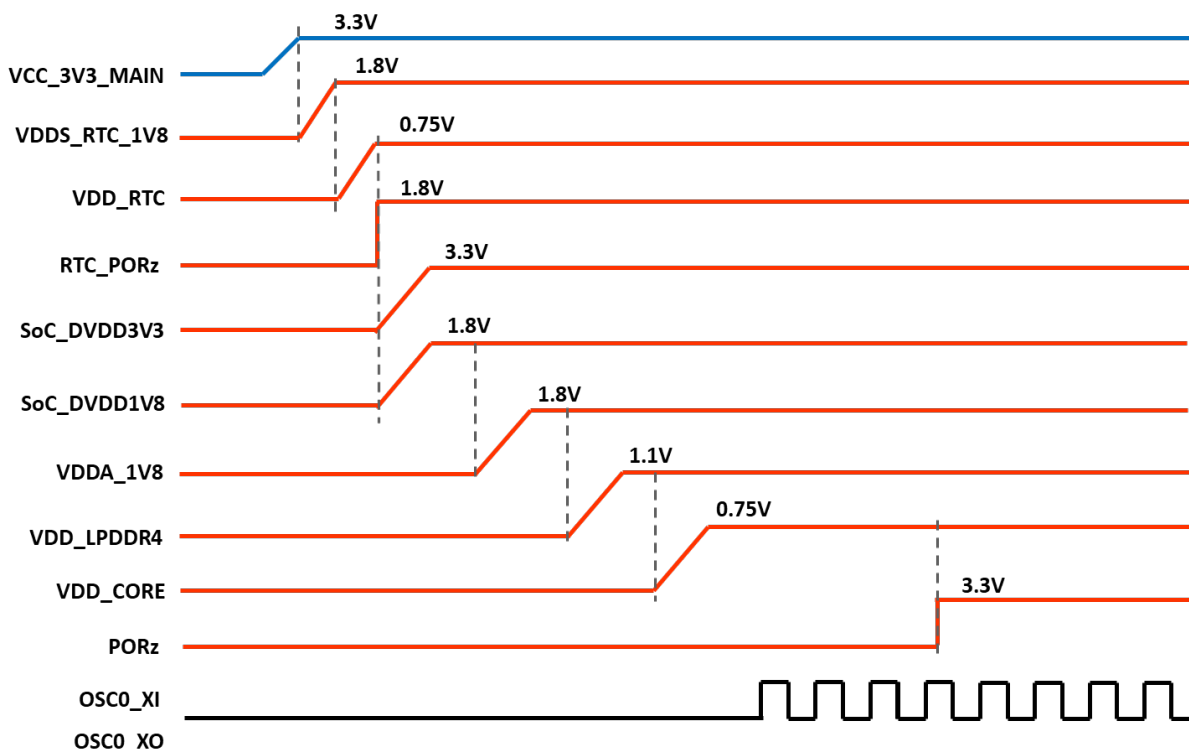
Figure 2-32. Power Sequence
