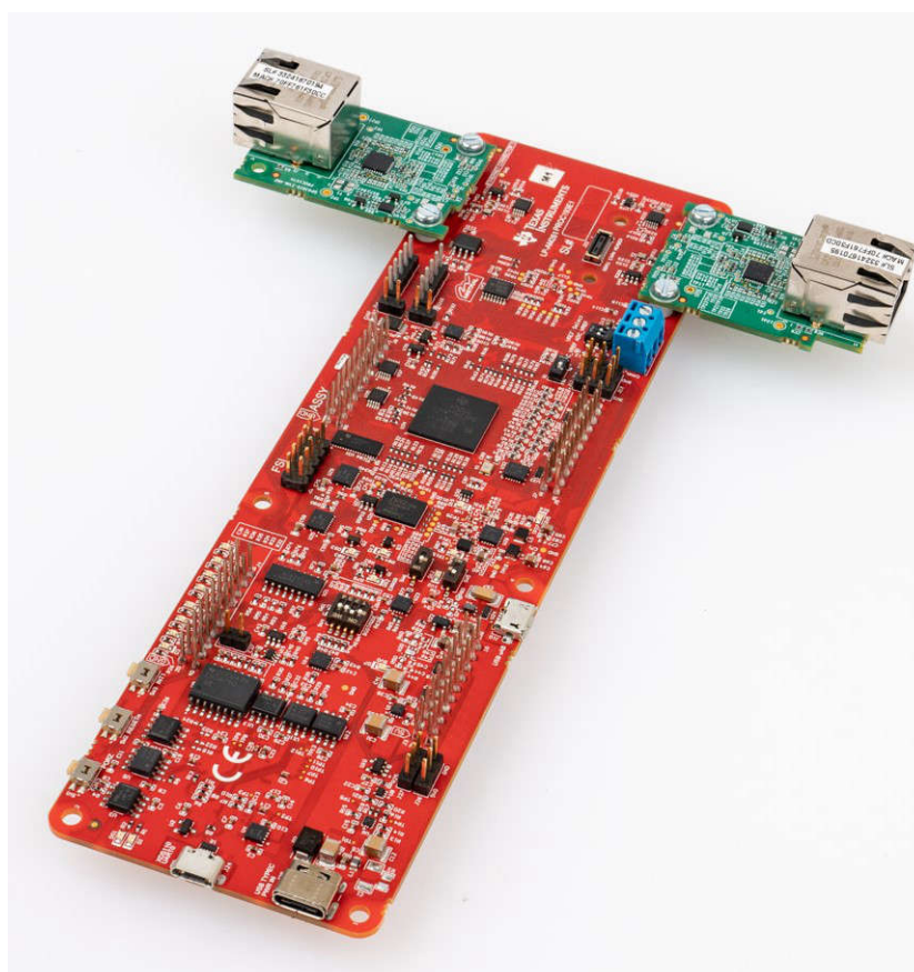
Figure 2-19. LP-AM261 with DP83826-EVM-AM2 Ethernet Add-on Boards
