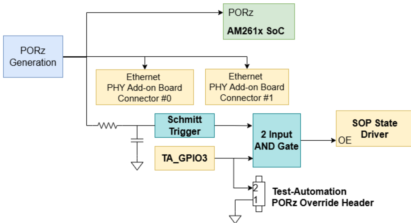
Figure 2-8. PORz Reset Signal Tree
