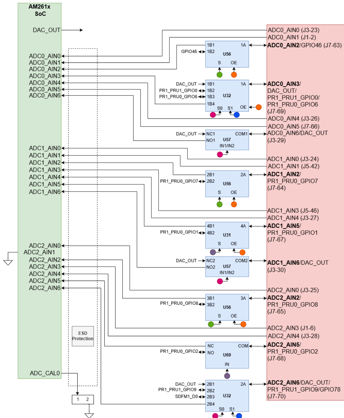
Figure 2-31. ADC/DAC Interface
