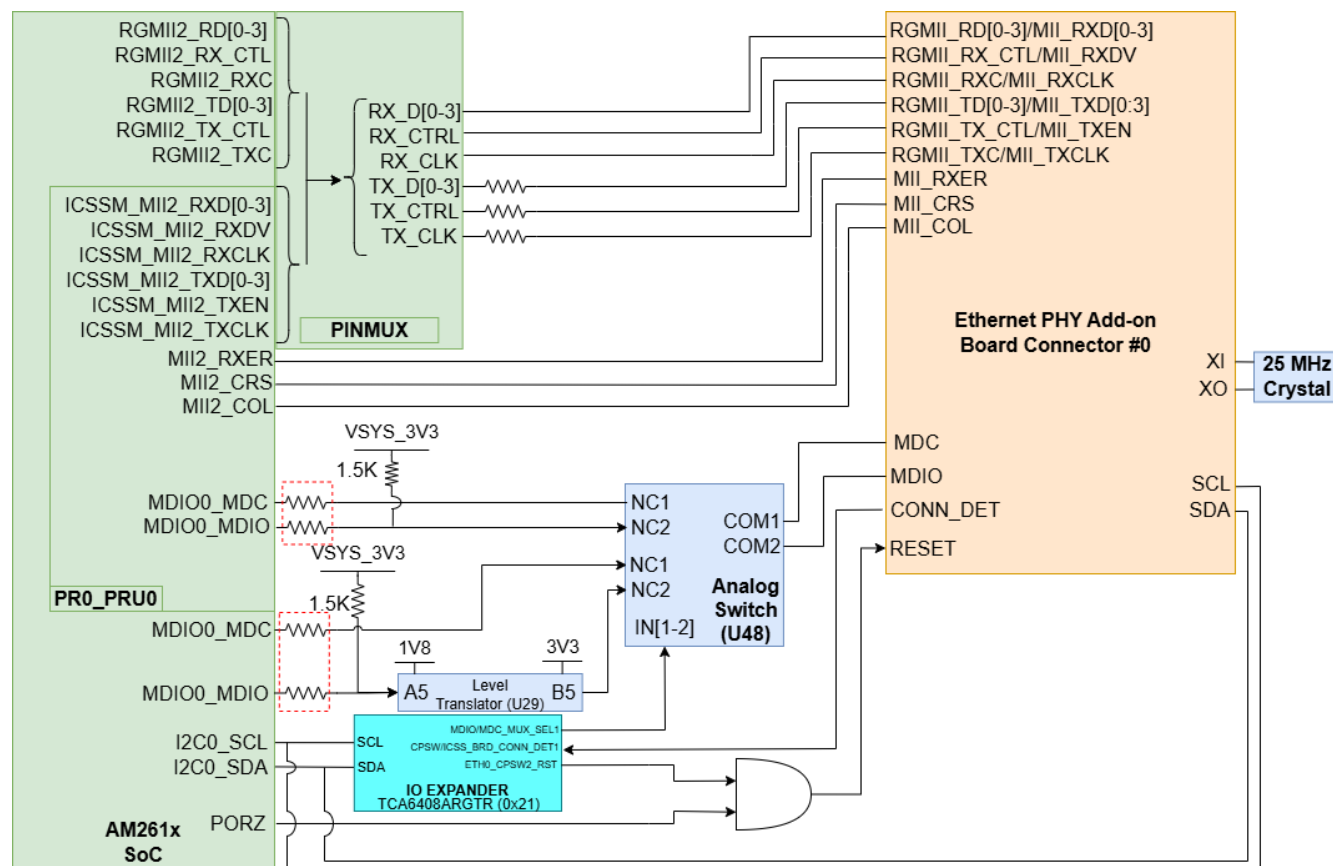
Figure 2-20. Ethernet PHY Add-on Board CONNECTOR_0
