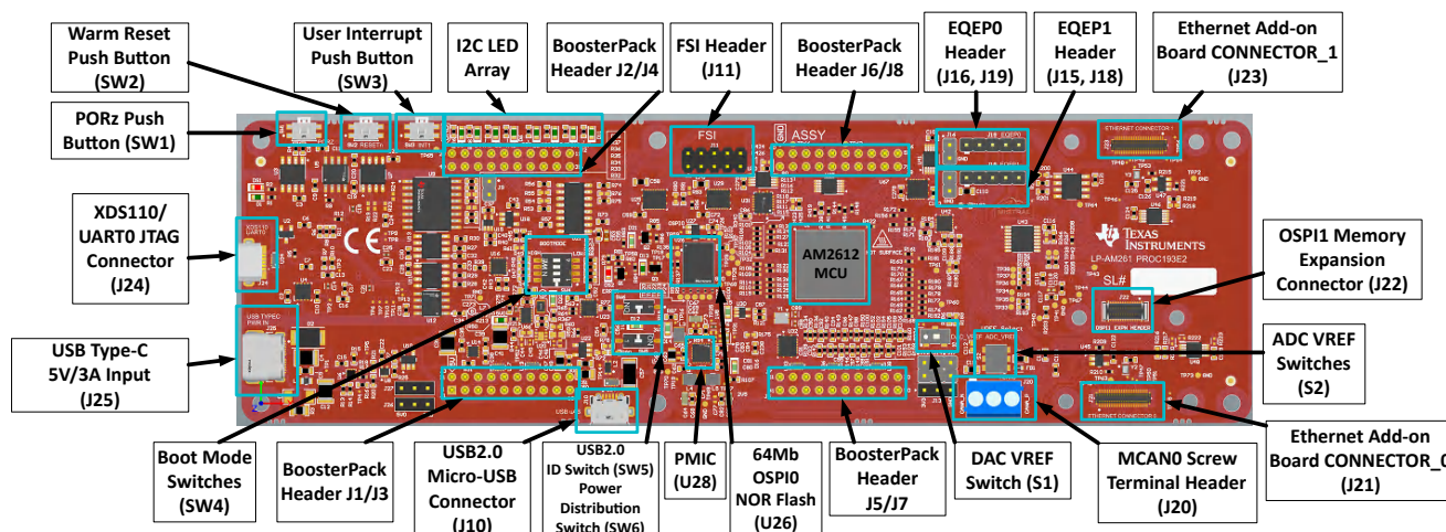
Figure 1-2. AM261x LaunchPad Top Components Identification
