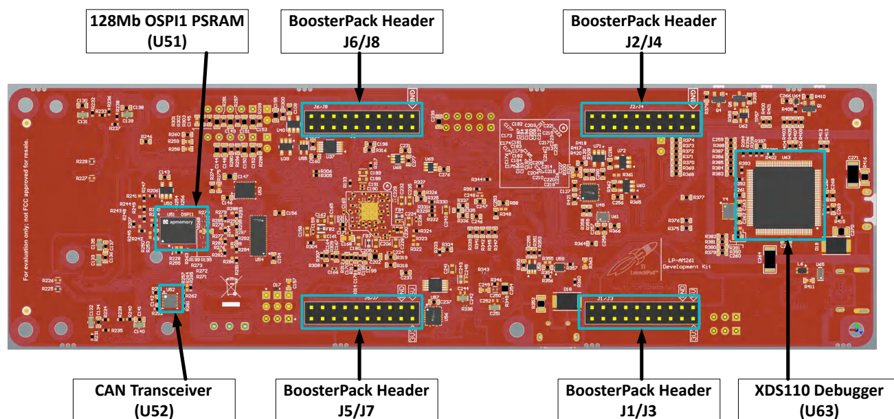
Figure 1-3. AM261x LaunchPad Bottom Components Identification
