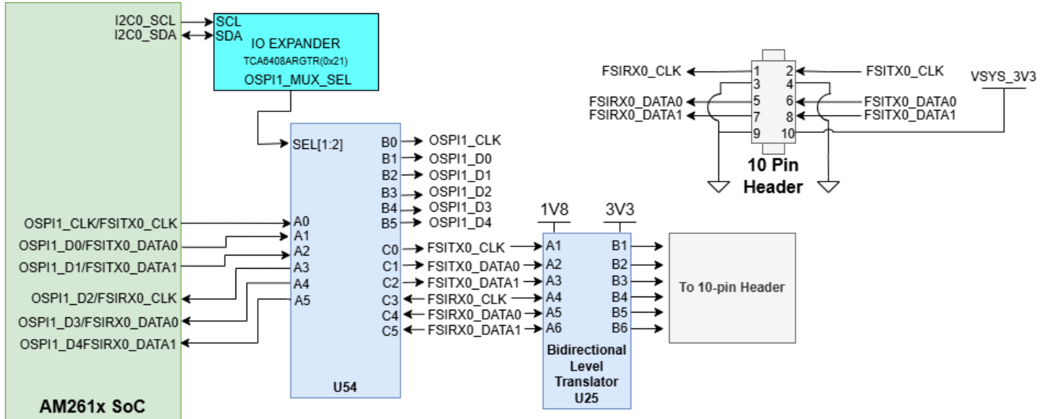
Figure 2-27. LP-AM261 FSI Interface
