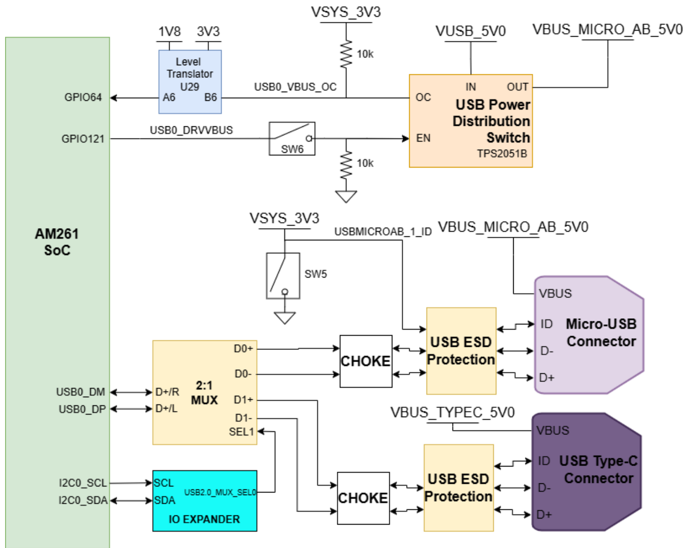
Figure 2-36. LP-AM261 USB Interface
