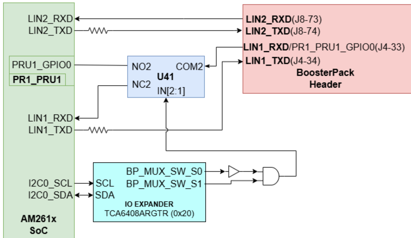
Figure 2-29. LIN Instances to BoosterPack Header
