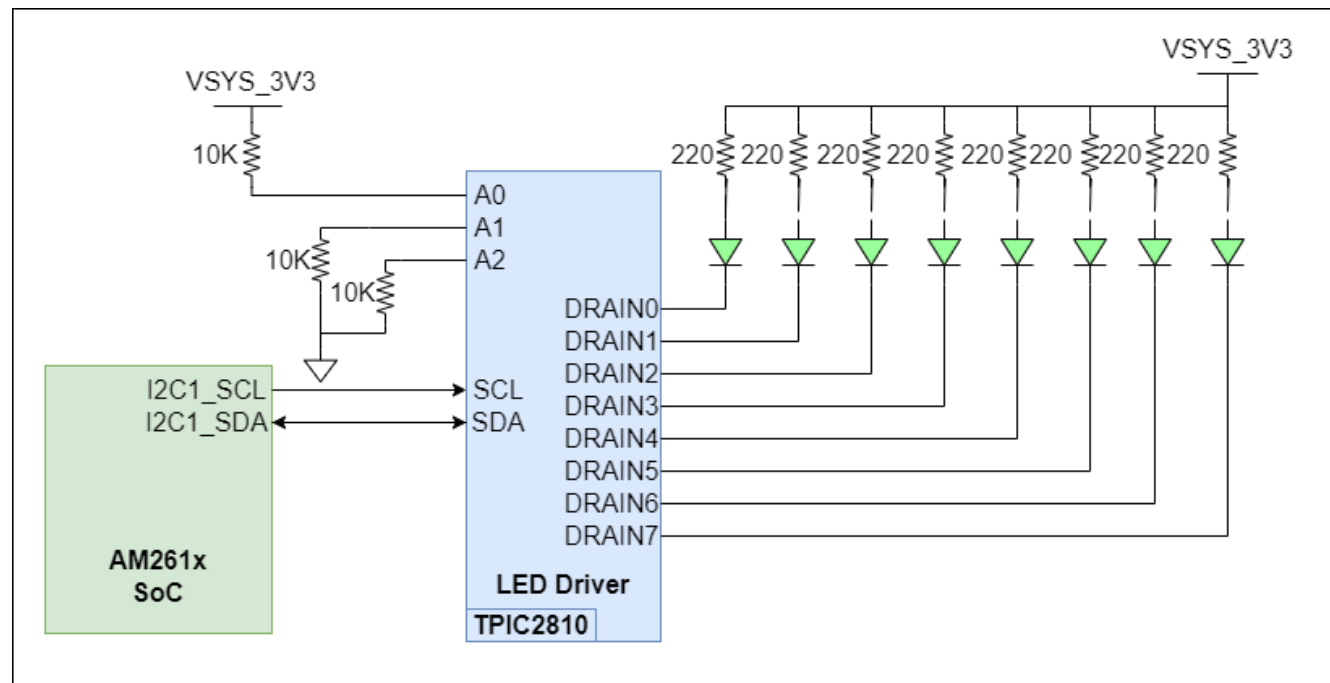
Figure 2-23. Industrial Application I2C LED Array
