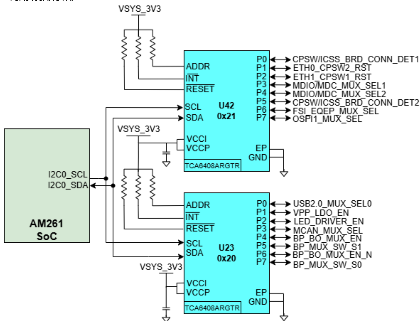
Figure 2-12. IO Expander
