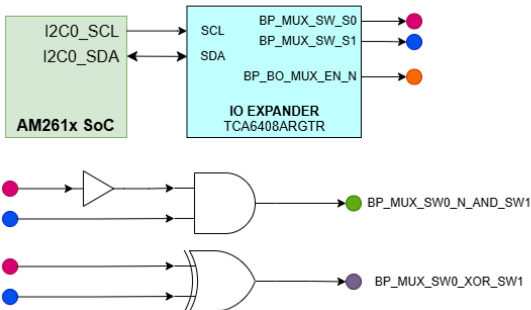
Figure 2-30. BoosterPack Mode Mux Select Logic
