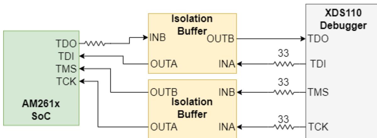
Figure 2-28. JTAG Interface to XDS110
