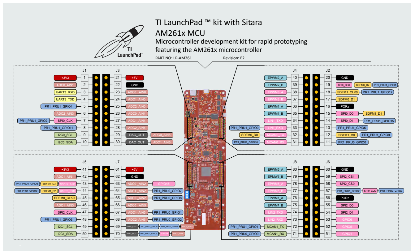
Figure 2-38. AM261x LaunchPad BoosterPack Pinout
