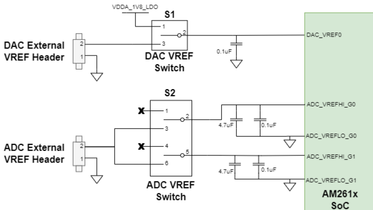
Figure 2-32. ADC and DAC VREF Switches
