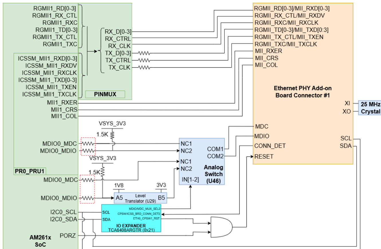
Figure 2-21. Ethernet PHY Add-on Board CONNECTOR_1
