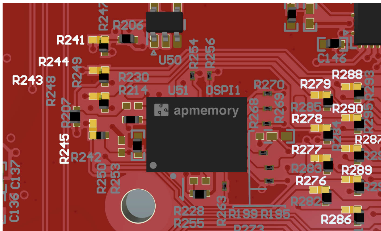
Figure 2-14. OSPI1 Expansion Connector - Populate Resistors
