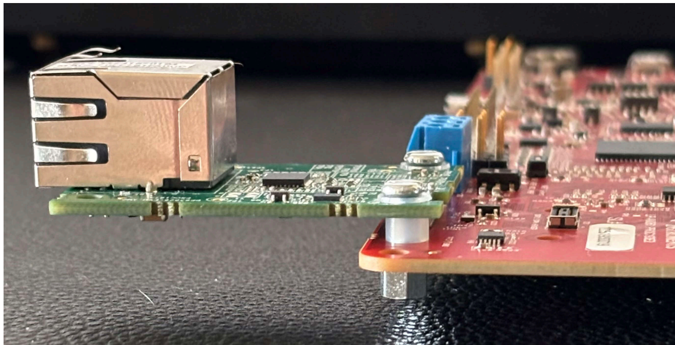
Figure 2-18. LP-AM261 and Ethernet Add-on Board Stack
