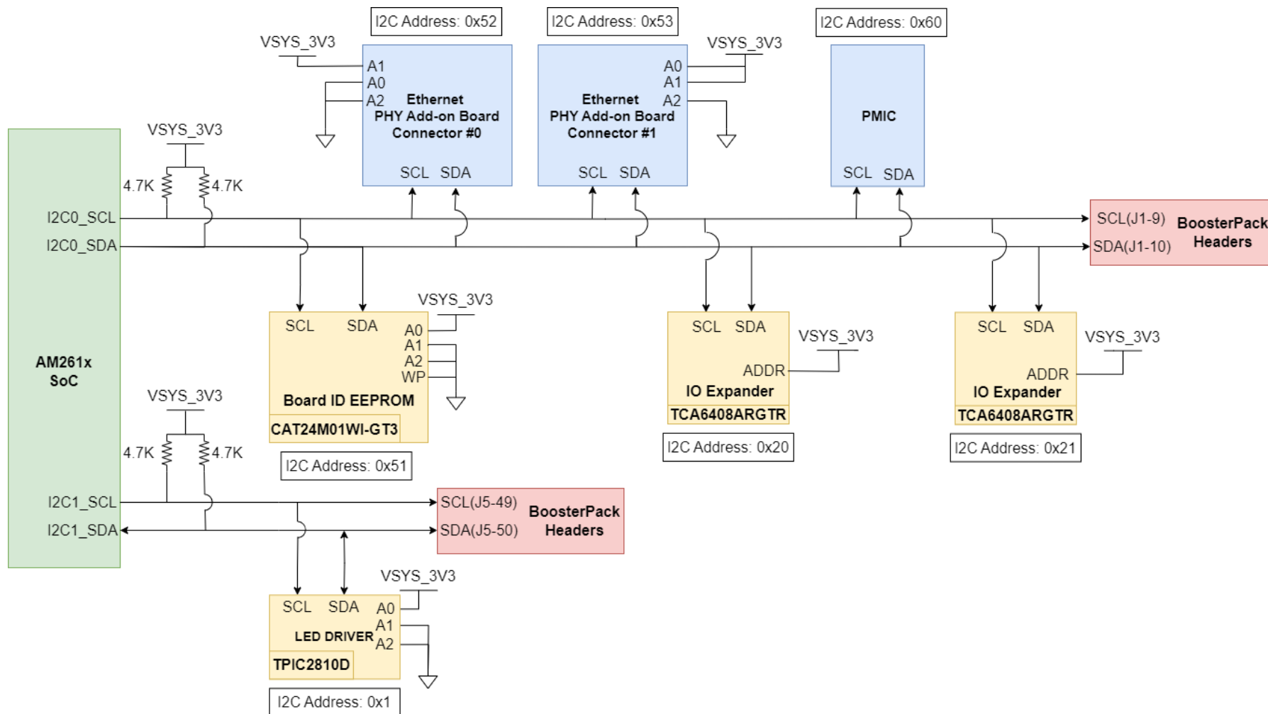
Figure 2-22. LP-AM261 I2C Interface
