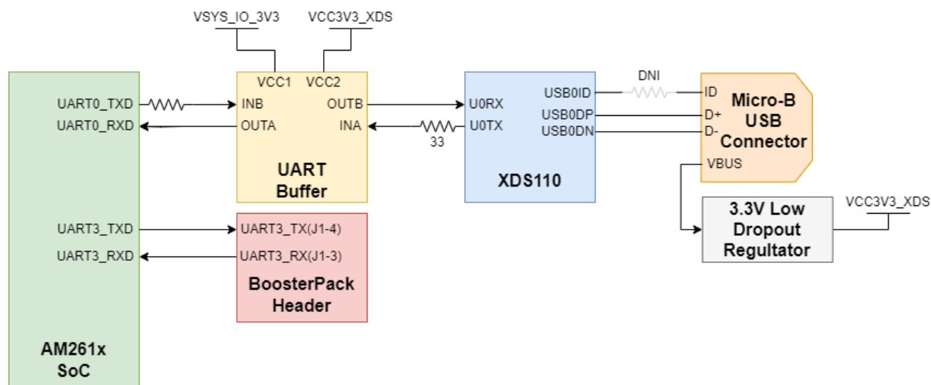
Figure 2-25. LP-AM261 UART Interface
