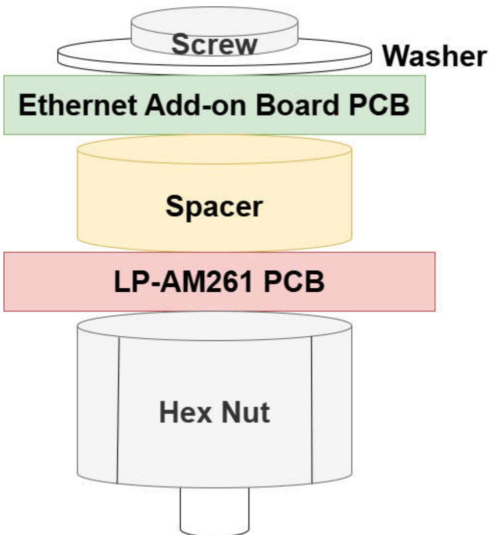
Figure 2-17. Ethernet Add-on Board Assembly Hardware
