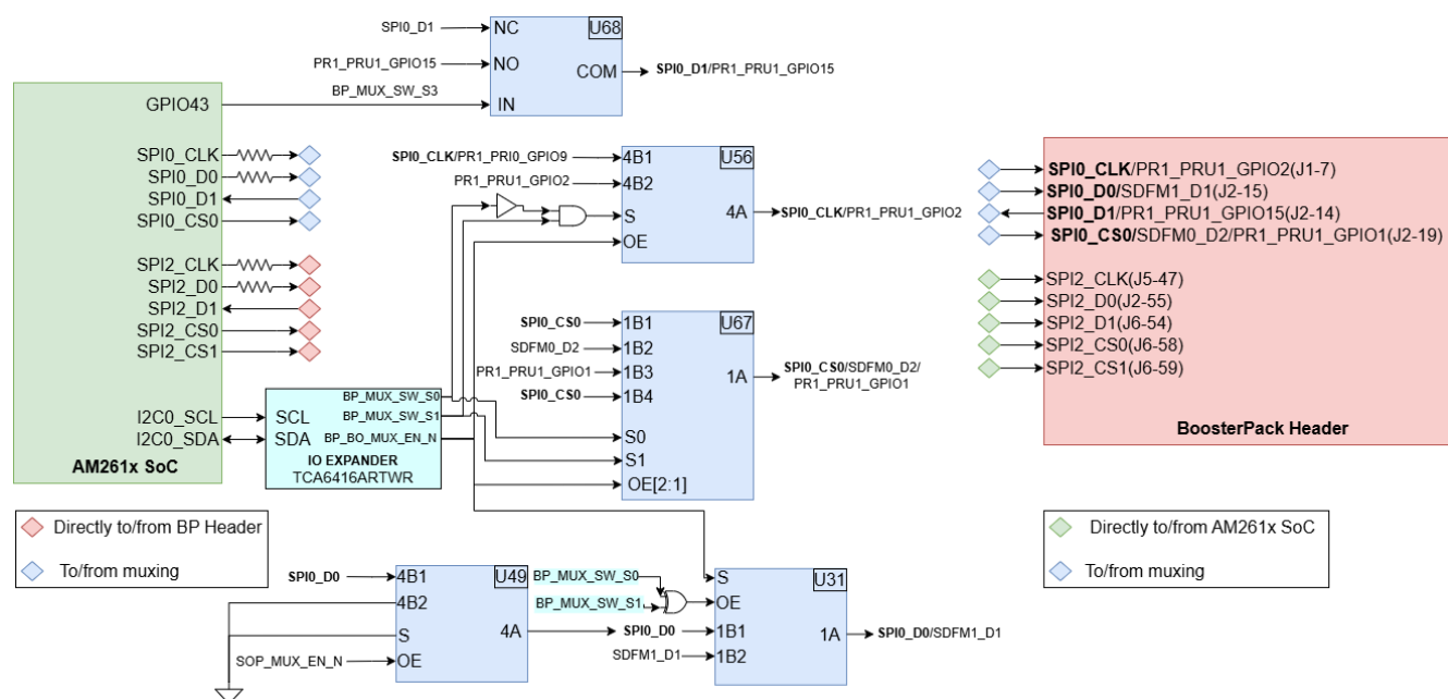
Figure 2-24. LP-AM261 SPI Interface
