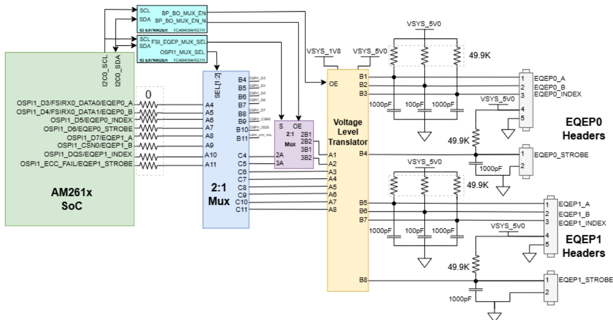
Figure 2-34. EQEP Signal Mapping
