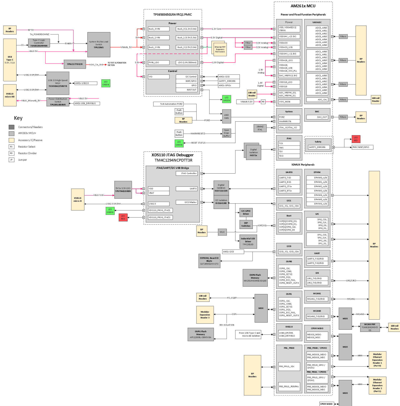
Figure 1-4. AM261x LaunchPad Functional Block Diagram
