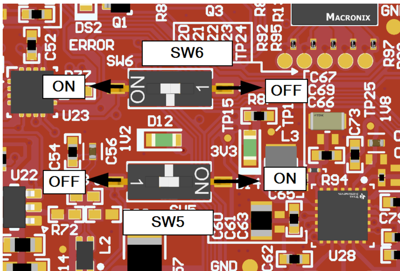
Figure 2-37. USB Mode Switches
