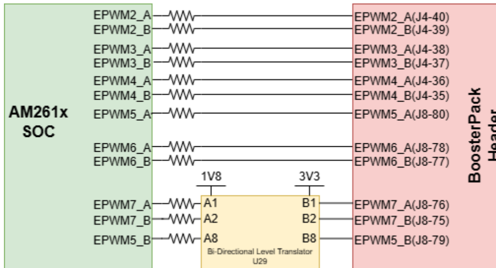
Figure 2-35. EPWM Signal Mapping to BoosterPack Header
