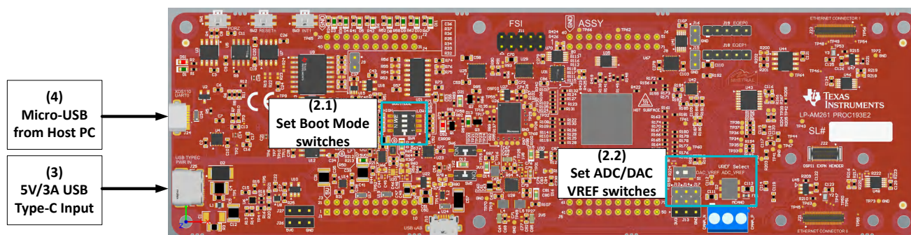
Figure 2-1. LP-AM261 Standalone Configuration
