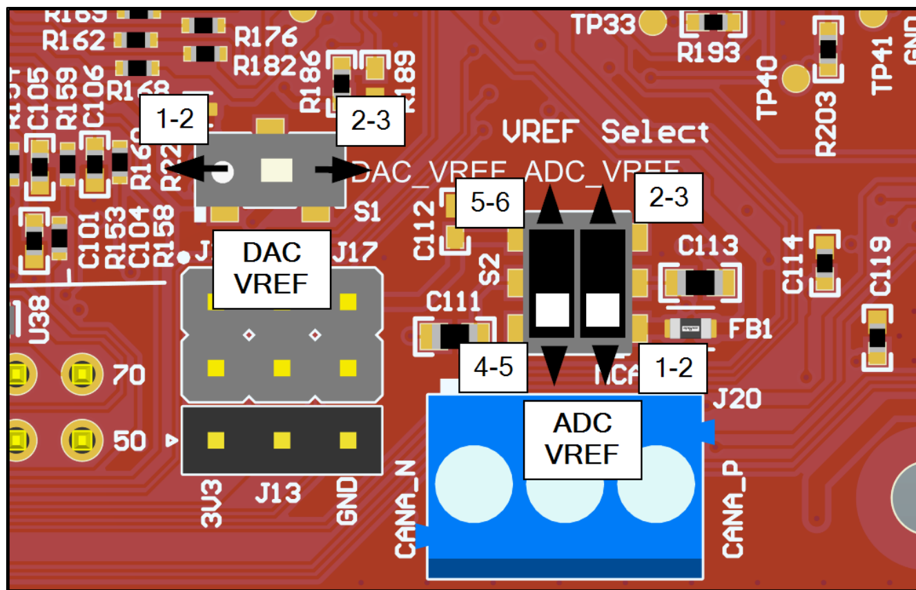
Figure 2-33. LP-AM261 ADC/DAC VREF Switches
