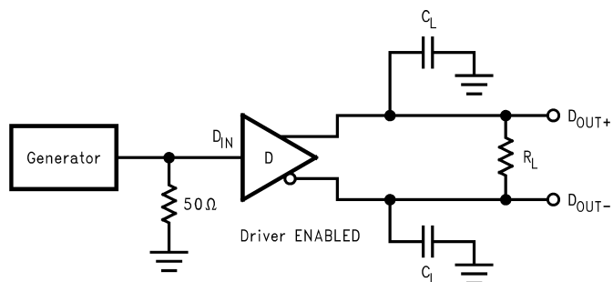
Figure 18. Driver Propagation Delay and Transition Time Test Circuit
