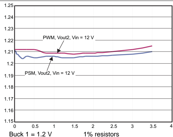
Figure 2. Load Regulation
