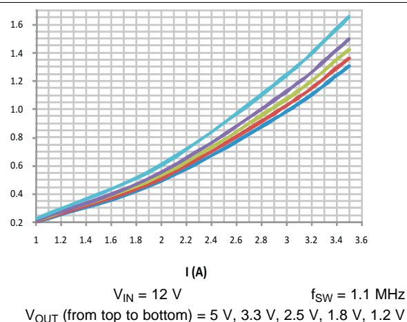
Figure 22. Buck 2
