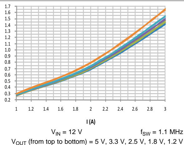
Figure 20. Buck 1
