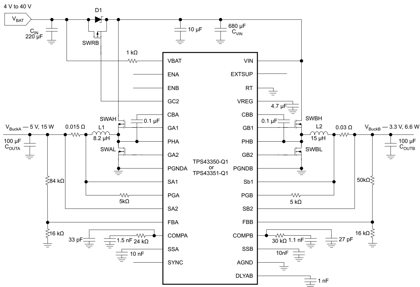
Figure 14. Simplified Application Schematic Example
