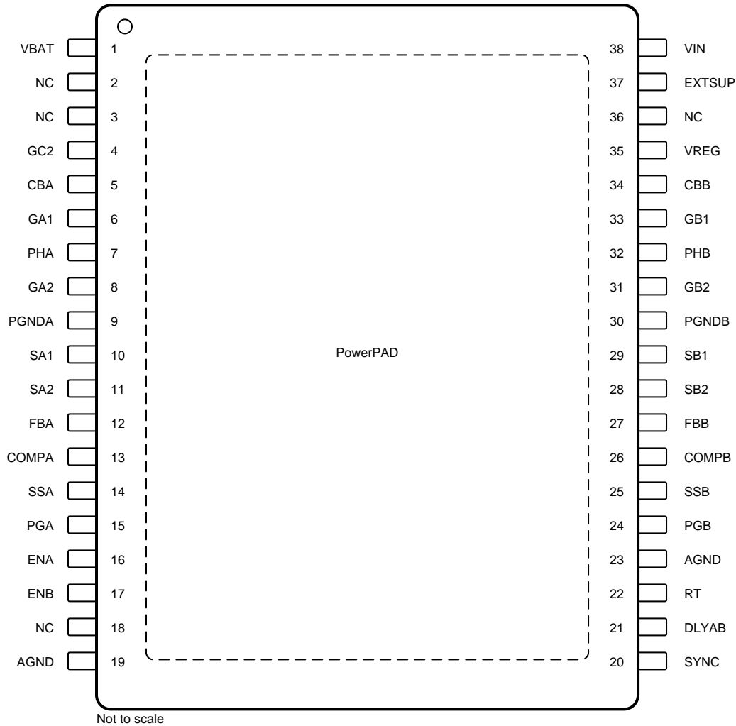
Pin Functions
