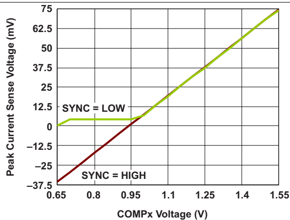
Figure 6. BUCKx Peak Current Limit vs COMPx Voltage
