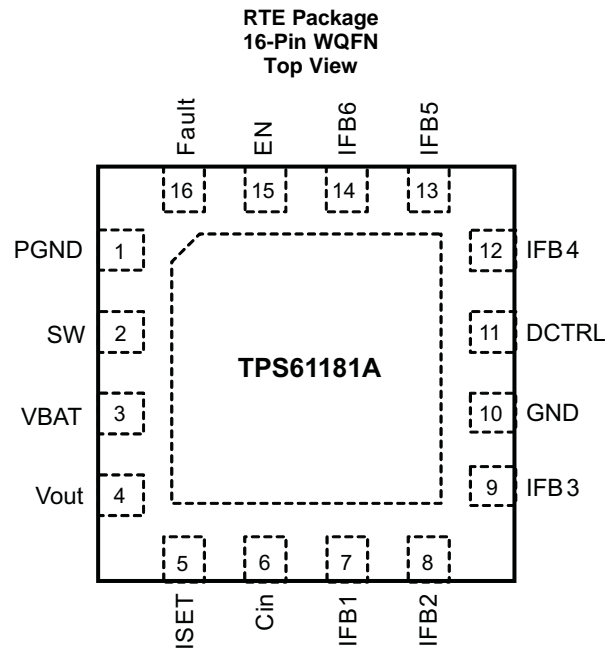
Pin Functions
