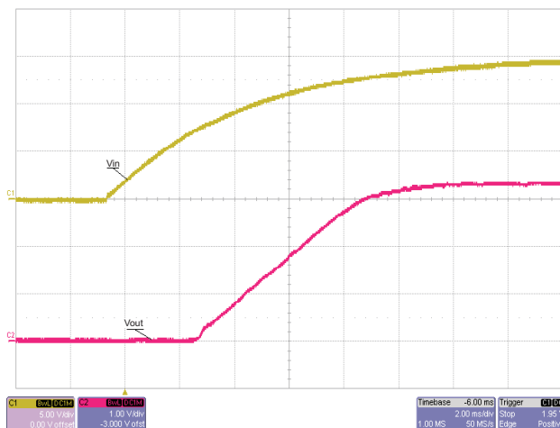
Figure 19. Startup
