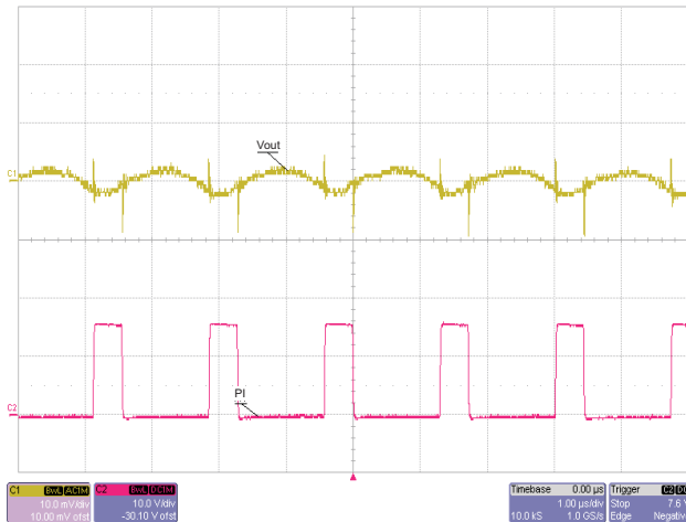
Figure 17. Output Ripple
