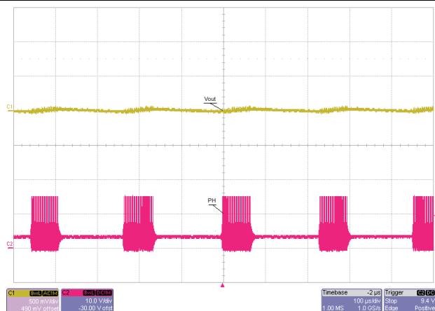
Figure 21. Eco-mode
