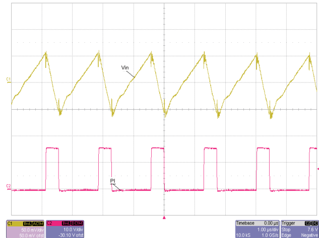
Figure 18. Input Ripple
