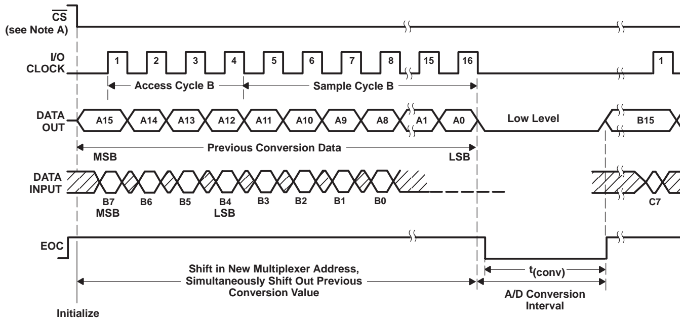
Figure 13. Timing for 16-Clock Transfer Using \overline{\text{CS}} With MSB First
