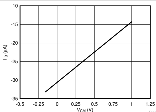
Figure 5-5. Input Bias Current vs Common-Mode Input Voltage
