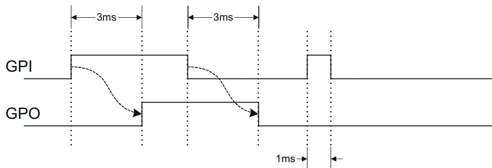
图 7-15. GPO Behavior When Not Ignoring Inputs During Delay
