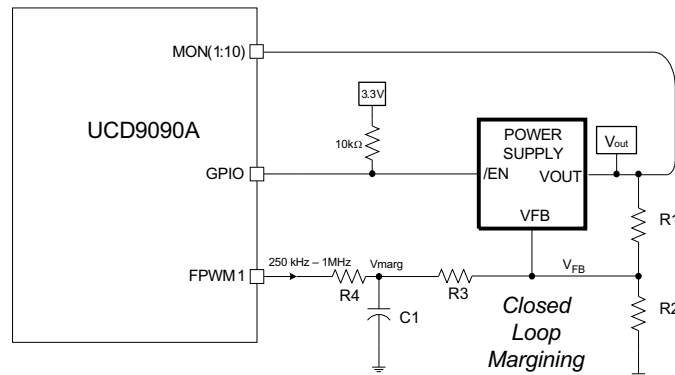
图 7-22. Closed-Loop Margining
