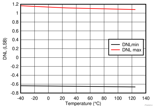
图 6-4. ADC Differential Nonlinearity vs Temperature
