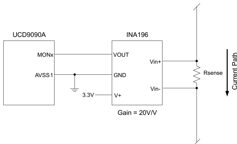
图 7-8. Current Monitoring Circuit Example Using the INA196
