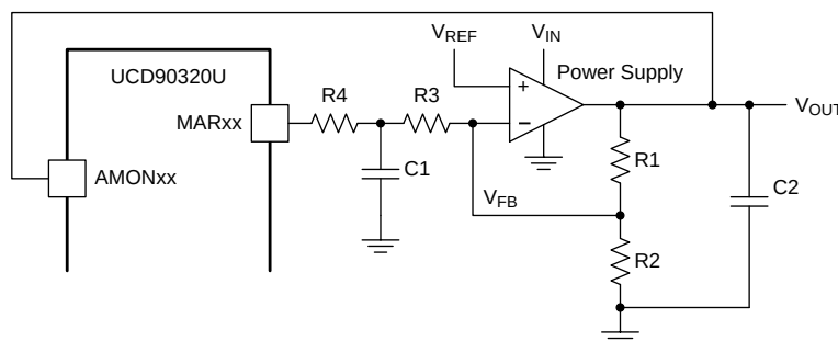
Figure 22. Block Diagram of Margining Circuit
