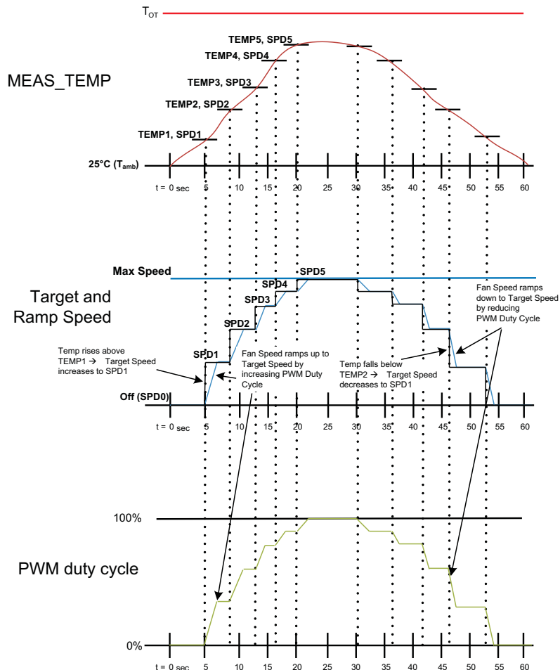
Figure 29. Temperature and Speed Set Point PWM Control for Four-Wire Fans
