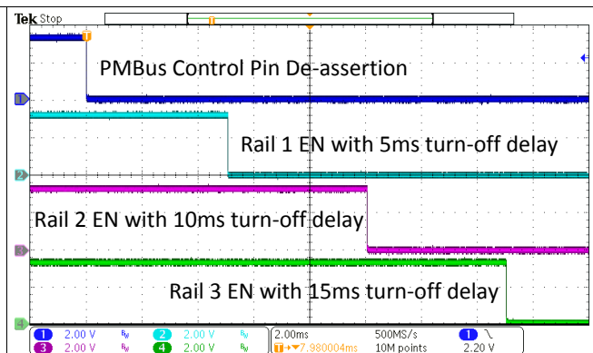
图 34. Example Power-off Sequence
