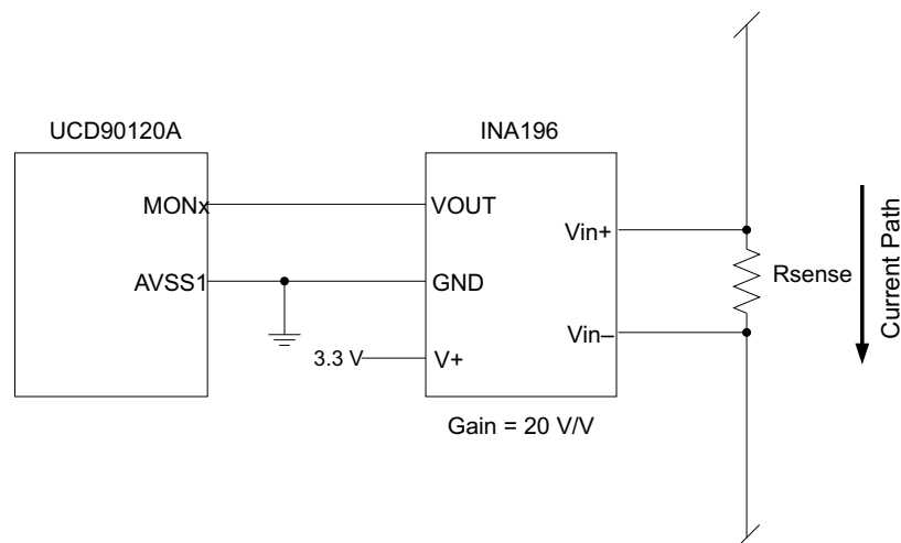
图 13. Current Monitoring Circuit Example Using The INA196
