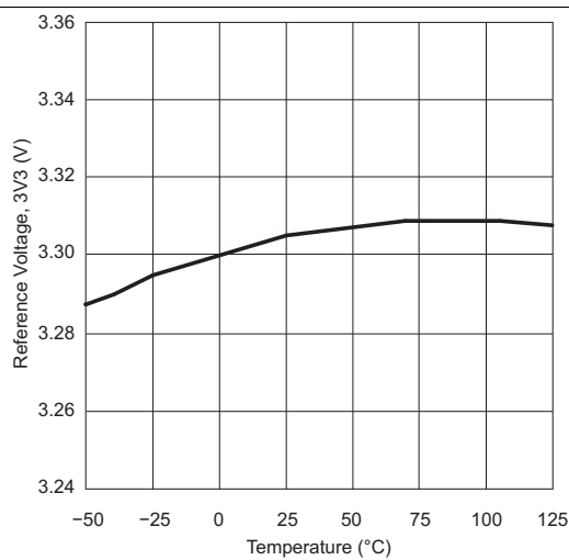
Figure 4. 3V3 Reference Voltage vs Temperature
