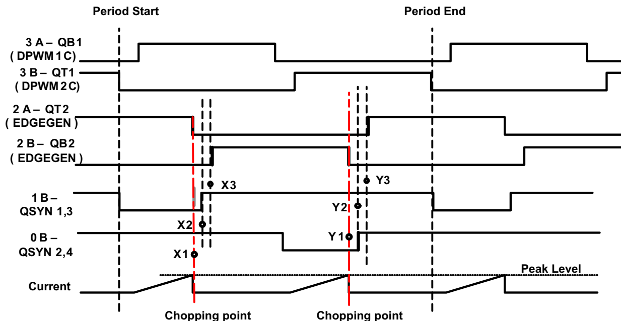
Figure 43. Final 6 Gate Signals
