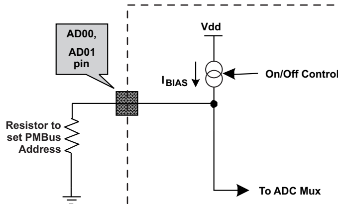
Figure 6-18. PMBus Address Detection Method
