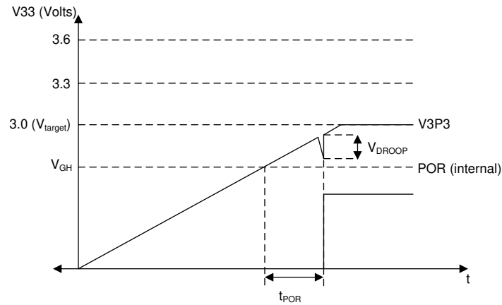
图 11-1. V33 Voltage Dip When POR is Activated
