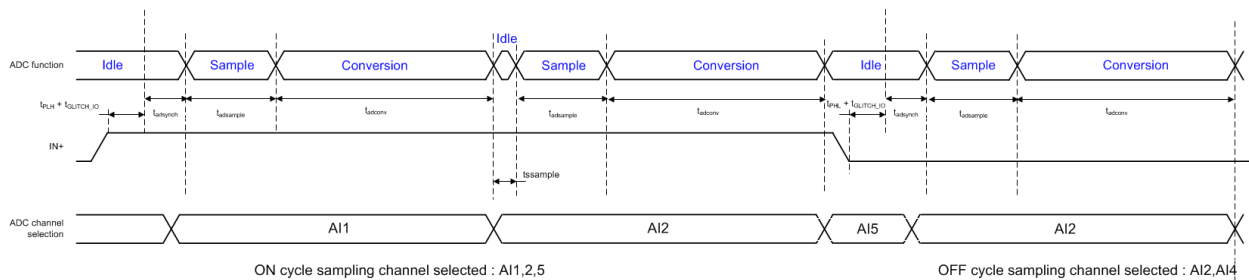
图 7-7. ADC Edge sampling mode timing chart
