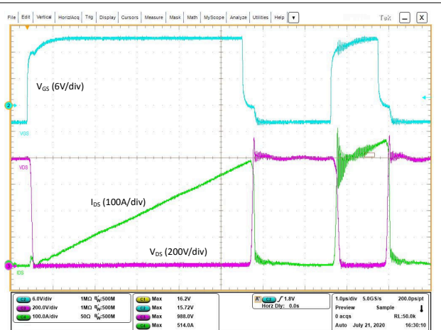
图 8-5. SiC Double Pulse Waveform
