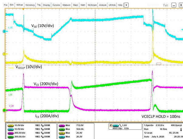
图 8-6. VCE Clamp Response with 100ns Hold Time
