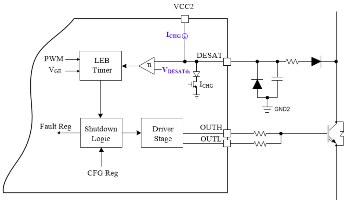
图 7-16. Block diagram of implementation of DESAT protection function.
