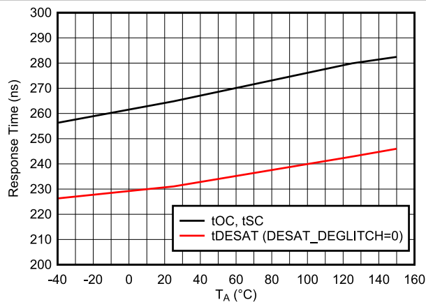
图 6-17. Overcurrent Protection Response Time vs. Temperature
