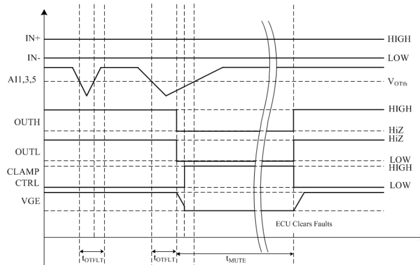
图 7-21. Timing scheme of implementation of PS_TSD function.
