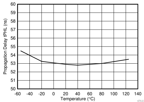
图 6-17. Propagation Delay t_{PHL} vs Temperature
