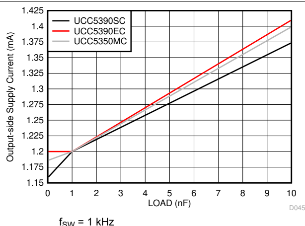
图 6-23. I_{CC2} Supply Current vs Load Capacitance
