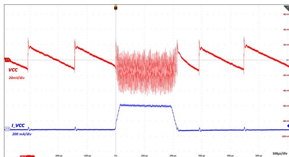
图 6-15. 负载瞬态: VINP = 5.0V, VCC = 5.0V, C OUT2 = 22 μF, I VCC = 0mA - 300mA - 0mA
