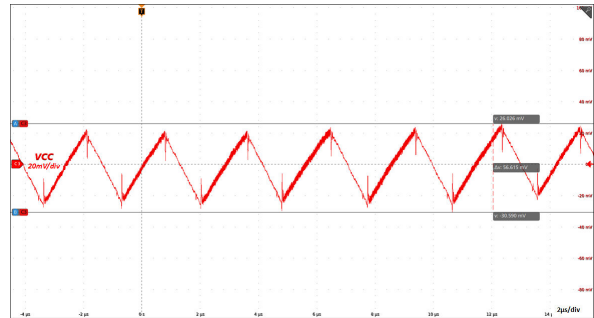
图 6-14. 稳态输出电压纹波: VINP = 5.0V, VCC = 5.0V, 300mA 负载
