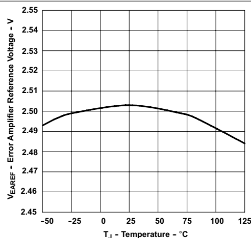
图 7-6. Error Amplifier Reference Voltage vs Temperature
