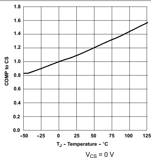
图 7-4. COMP to CS Offset Voltage vs Temperature
