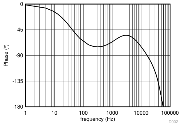
图 9-4. Converter Open-Loop Bode Plot - Phase
