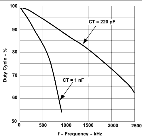
图 7-15. Maximum Duty Cycle vs Oscillator Frequency
