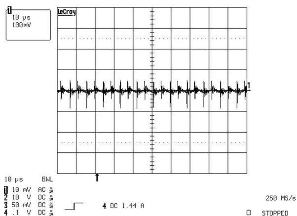
图 9-10. Output Voltage Ripple at Full Load (100 mV/div)
