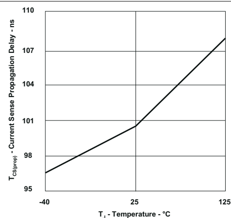
图 5-20. Current Sense Propagation Delay vs Temperature
