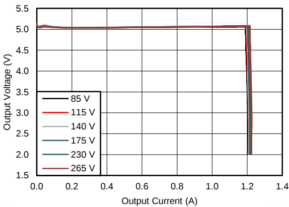
Figure 33. Output V-I Characteristic
