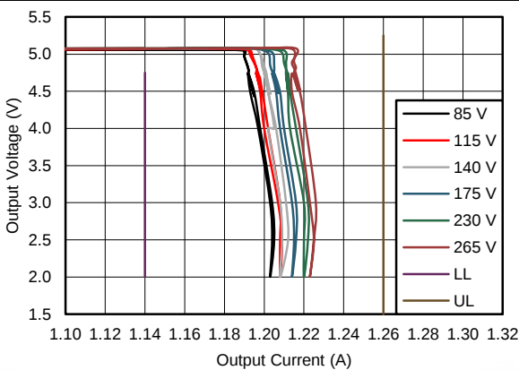
Figure 35. Output V-I Characteristic Output Voltage Regulation
