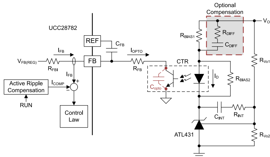
图 9-3. Compensation Network, H_v(s)
