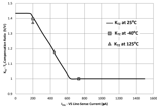
图 7-7. t_Z Compensation Ratio ( K_{TZ} ) vs. VS Line-Sense Currents
