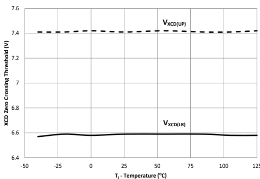
图 6-12. XCD Thresholds vs. Junction Temperature
