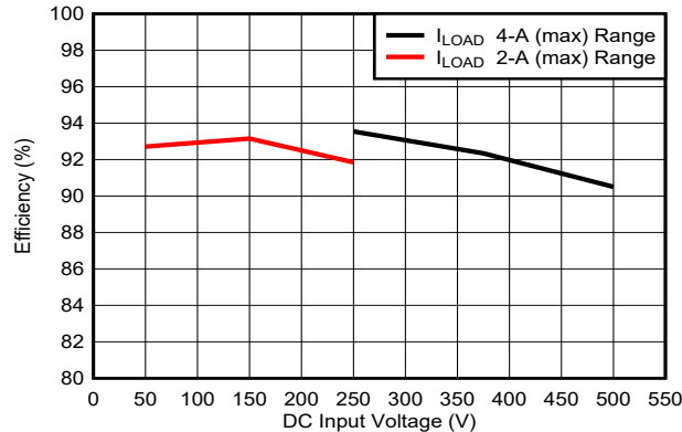
图 8-4. 4pt-Average Efficiency vs. DC Input Voltage
