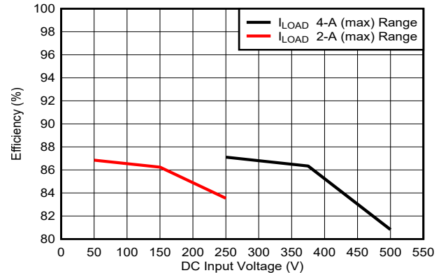
图 8-5. 10%-Load Efficiency vs. DC Input Voltage
