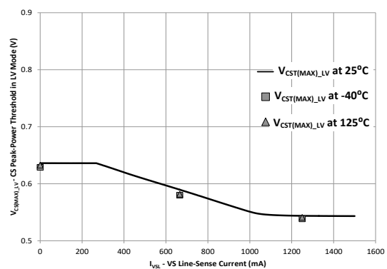
图 6-6. CS Peak-Power Threshold for V_{VS} < V_{VSLV(LR)} vs. VS Line-Sense Currents
