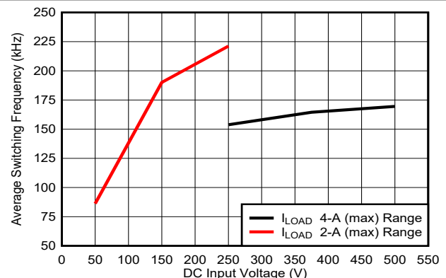
图 8-7. Average Switching Frequency at Full-Load vs. DC Input Voltage
