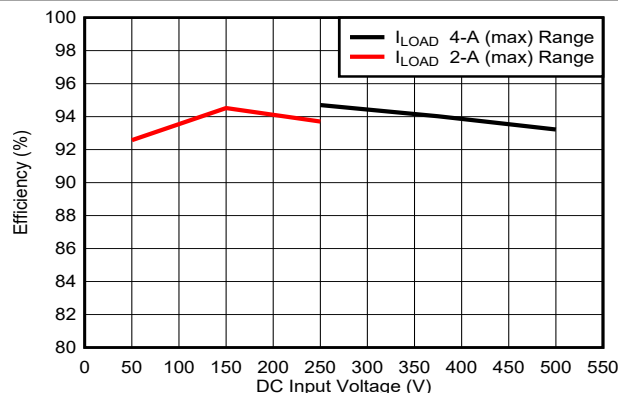
图 8-6. Full-Load Efficiency vs. DC Input Voltage
