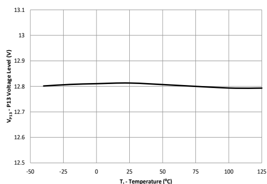
图 6-10. P13 Voltage vs. Temperature
