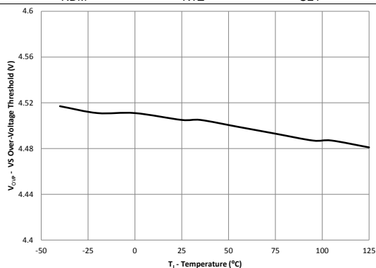
图 7. VS Over-Voltage Threshold vs. Temperature
