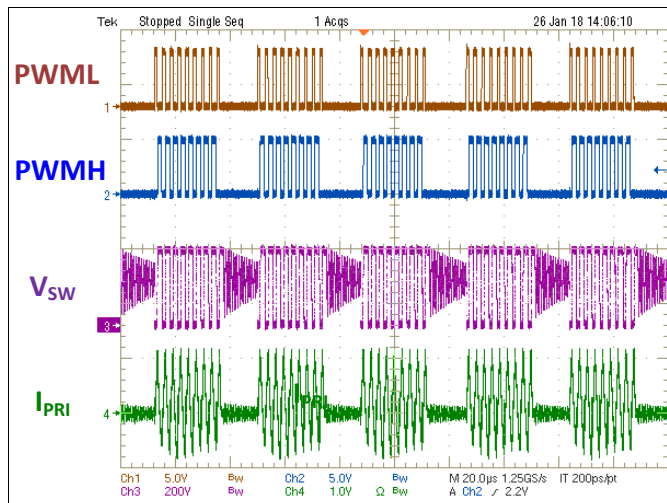
图 46. AAM Waveforms at V_{IN} = 230 V_{RMS} and I_O = 2.25 A
