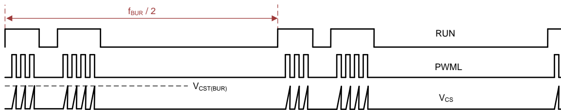
图 39. Typical Behavior of Unstable ABM Loop
