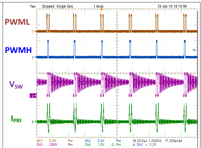
图 49. ABM Waveforms at V_{IN} = 115 V_{RMS} and I_O = 0.2 A
