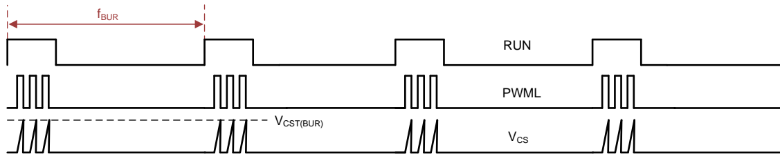
图 38. Expected Burst Pattern Example
