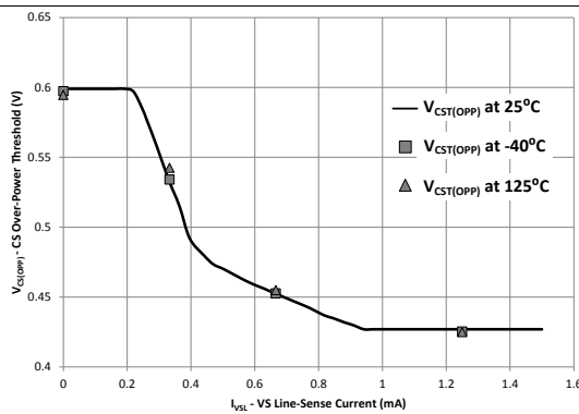
图 5. CS Over-Power Threshold vs. VS Line-Sense Currents
