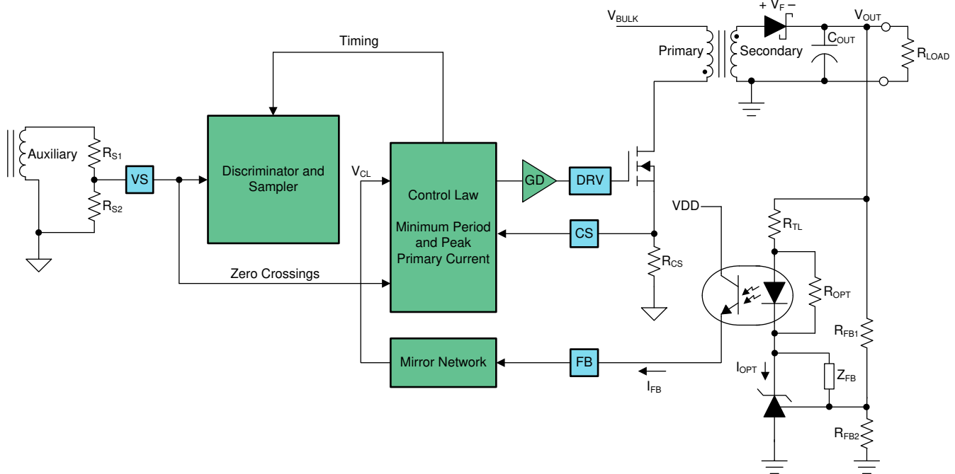
图 7-2. Simplified Flyback Convertor (With the Main Voltage Regulation Blocks)
