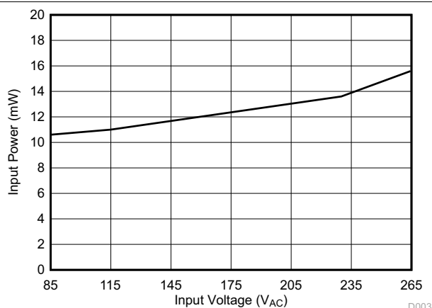
图 8-8. No Load Power Consumption
