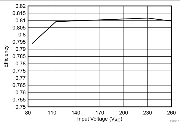
图 8-7. Average Efficiency
