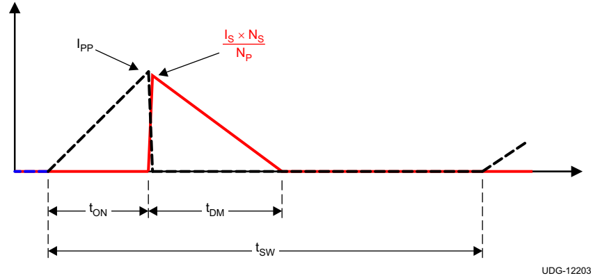
图 7-6. Transformer-Current Relationship
