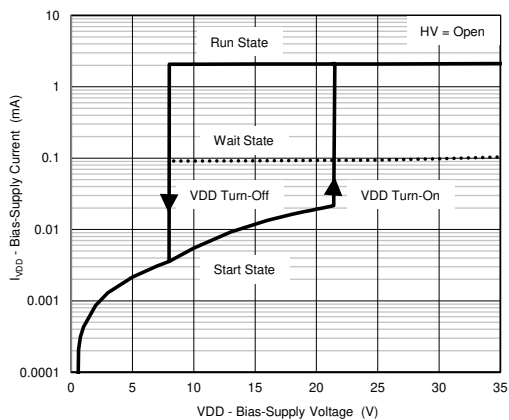
图 6-1. Bias-Supply Current vs. Bias-Supply Voltage
