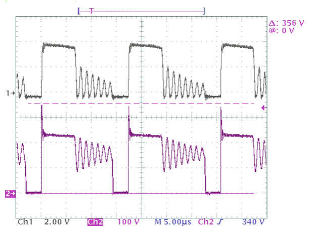
CH 1 = VS CH 2 = V DS I OUT = 1.8 A V IN = 115 VAC, 60 Hz
