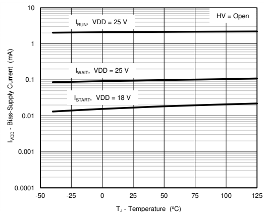
图 6-2. Bias-Supply Current vs. Temperature
