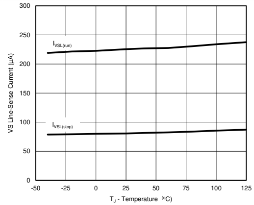
图 6-4. VS Line-Sense Currents vs. Temperature
