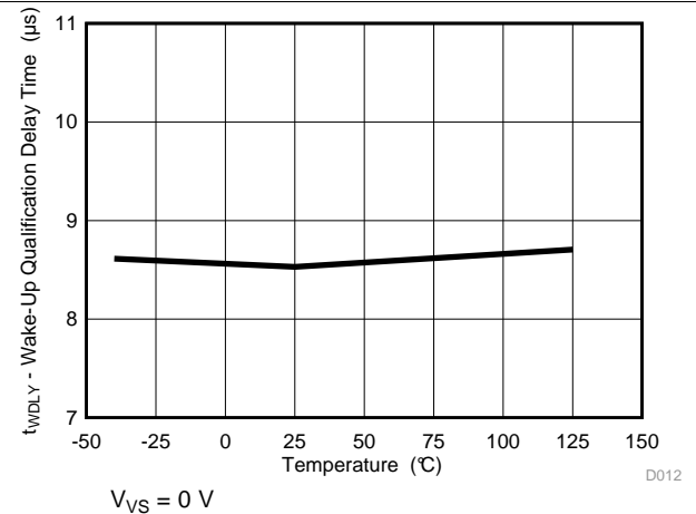
图 12. Wake-Up Qualification Delay Time vs. Temperature
