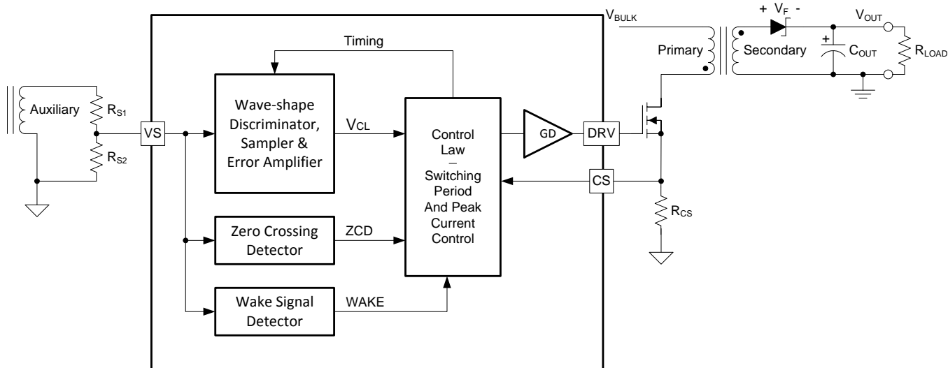
图 13. Simplified Flyback Convertor (with the main voltage regulation blocks)
