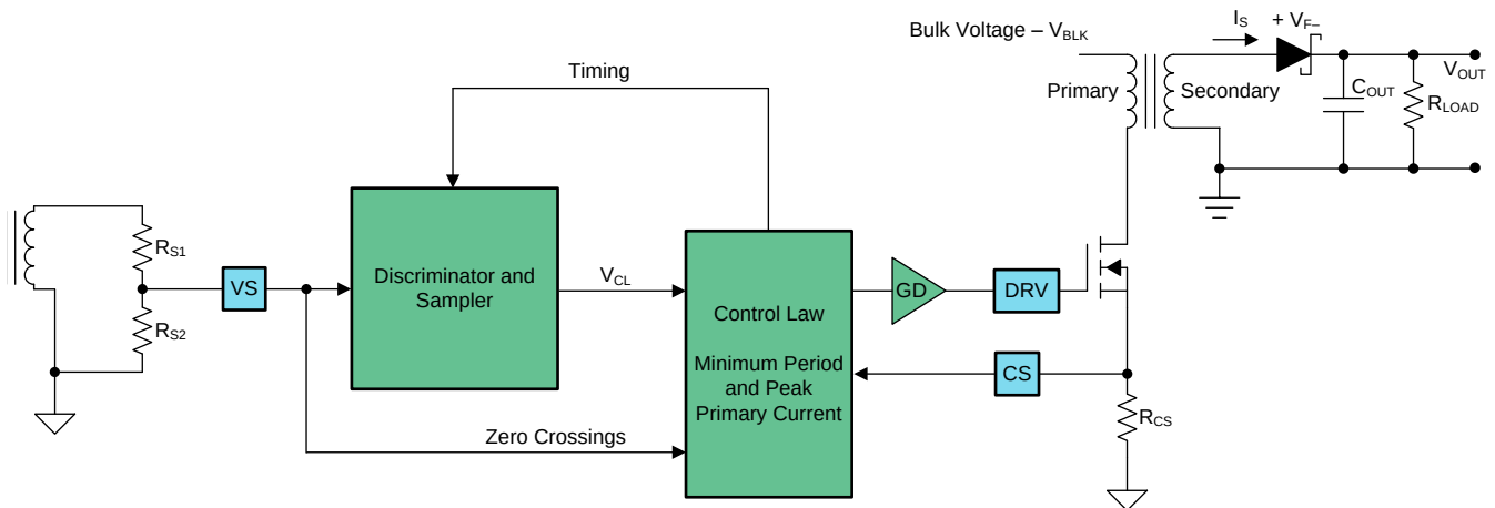
Figure 13. Simplified Flyback Convertor (With the Main Voltage Regulation Blocks)
