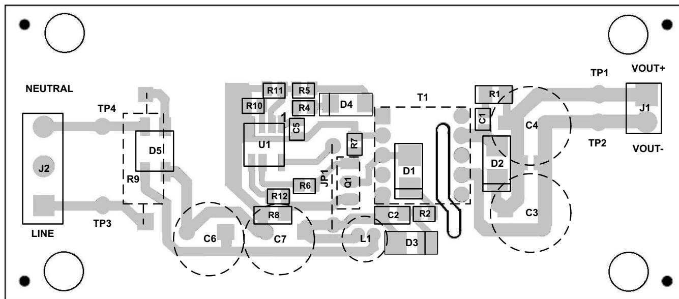
Figure 30. Layout Example Schematic
