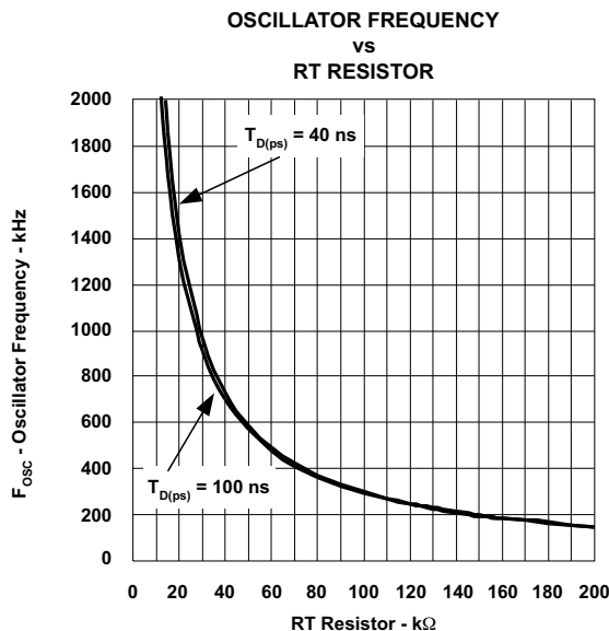
Figure 24. Oscillator Frequency F_{OSC} vs External Resistance of RT at T_{D(SP)} = 40 \text{ ns} and 100 \text{ ns}
