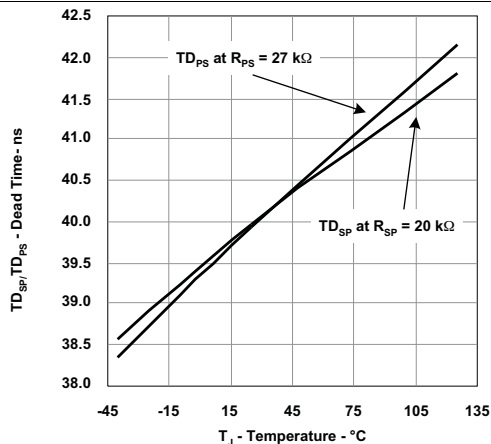
Figure 18. Dead Time vs Temperature
