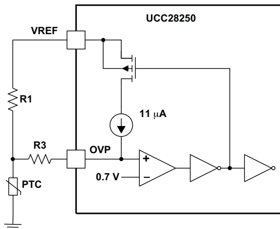
Figure 37. Overtemperature Protection
