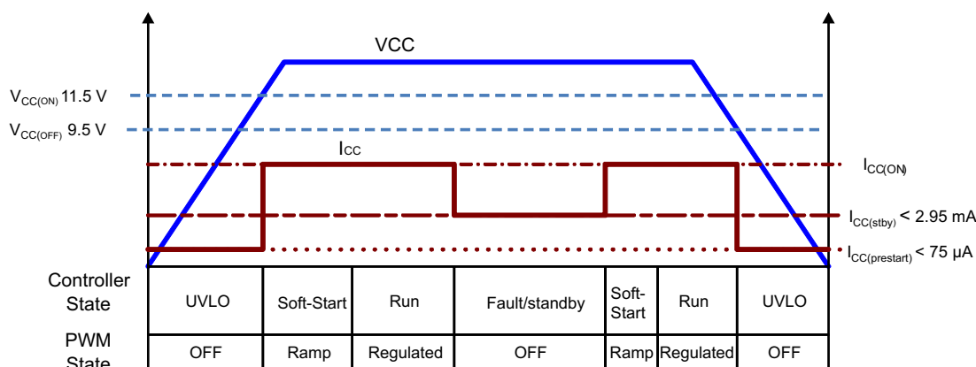
图 40. Device Supply States
