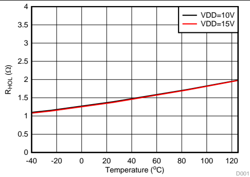
图 20. HO Output Pull-Down Resistance vs Temperature
