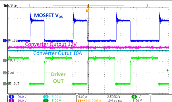
图 8-8. Output Voltage and Current of a Converter Using UCC27634DSG
