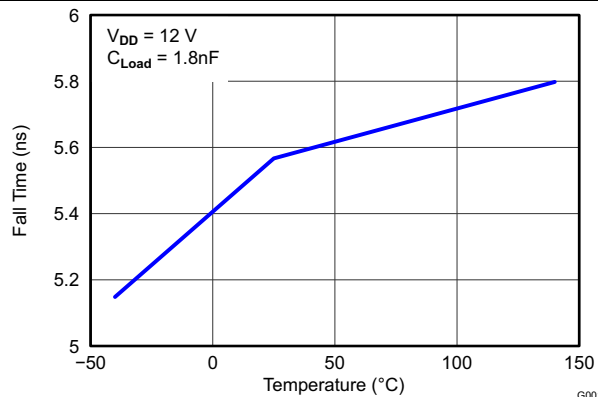
Figure 8. Fall Time
