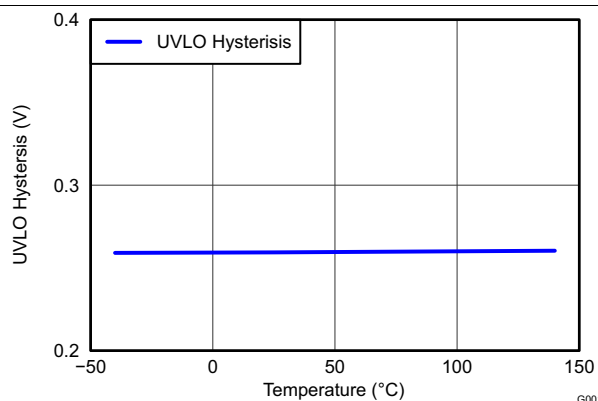
Figure 6. UVLO Hysteresis
