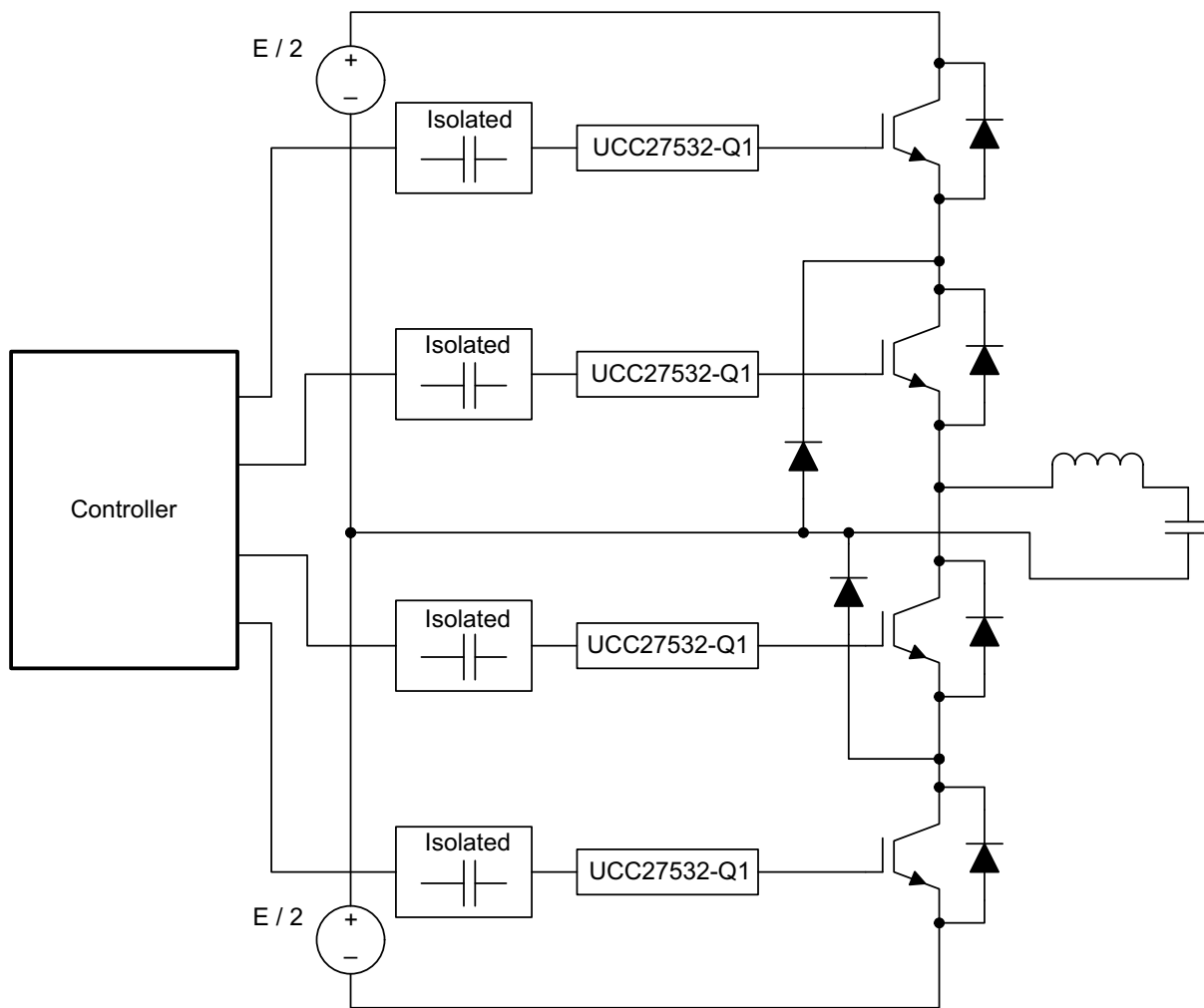
图 8-6. Using UCC27532-Q1 Drivers in an Inverter
