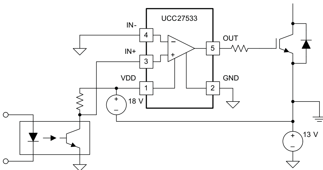
图 46. Single-Output Driver
