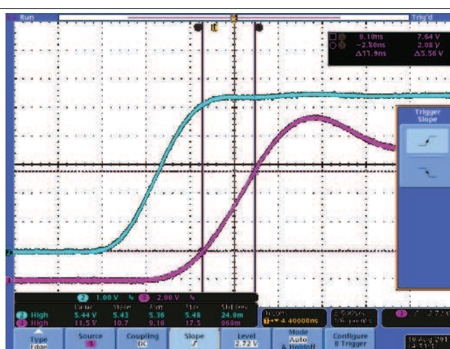
Figure 25. Typical Turnoff Waveform
